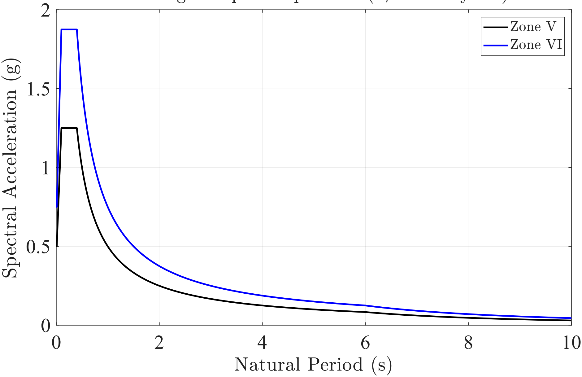
IS Design Response Spectrum ( T_r = 2475 years)
